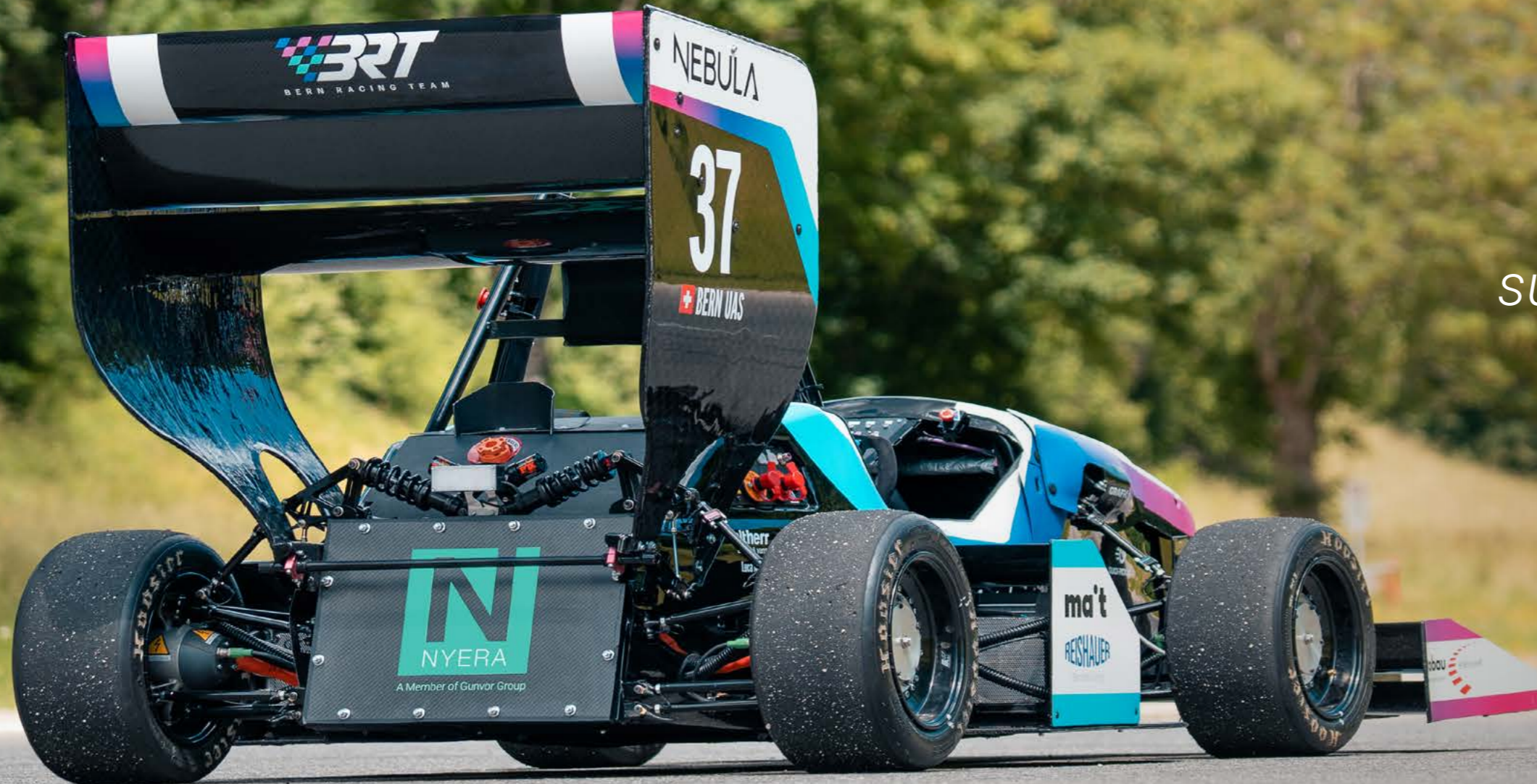
"Nebula" is a 4-wheel drive electric race car developed by the Bern Racing Team, sponsored by Nyera, Gunvor's renewables investment vehicle.
